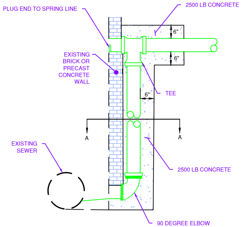
VERTICAL SECTION
