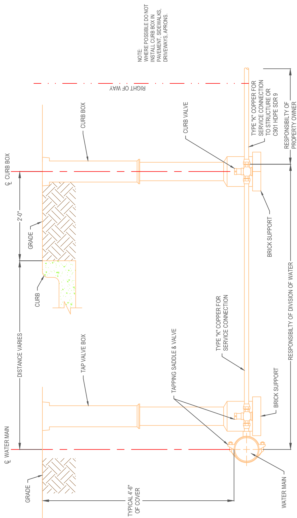
NEW WATER SERVICE CONNECTION FOR 1-1/2" & 2"
