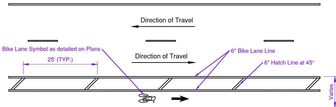
BIKE LANE BUFFER DETAIL
